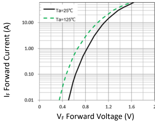
Figure 1. Forward Characteristic(typ.)
