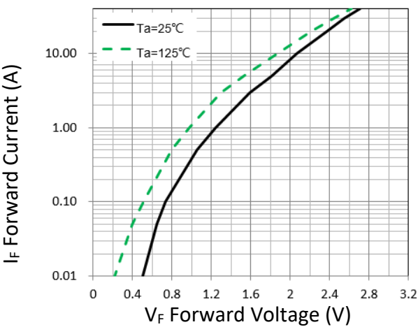
Figure 1. Forward Characteristic(typ.)
