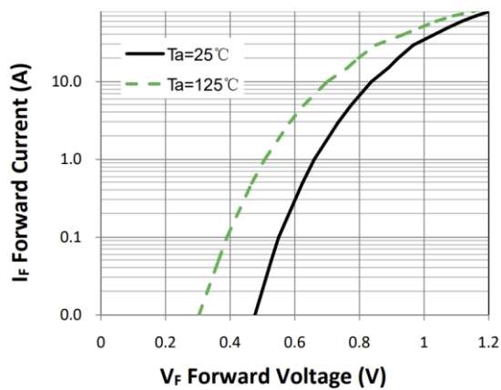
Figure 1. Forward Characteristic(typ.)
