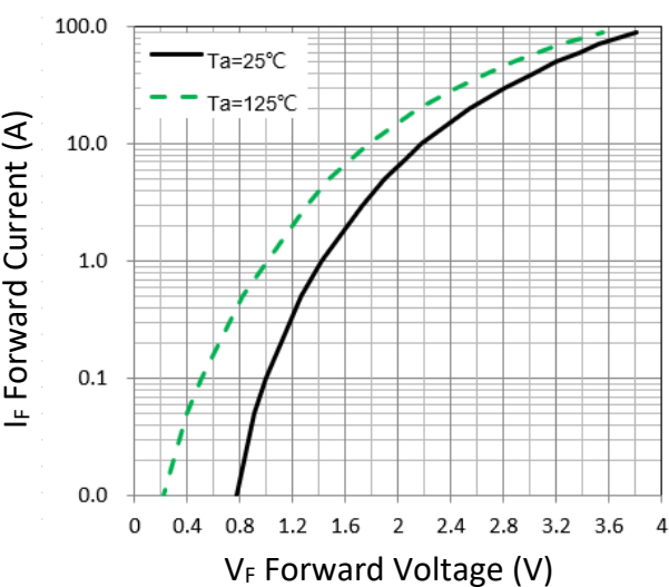
Figure 1. Forward Characteristic(typ.)
