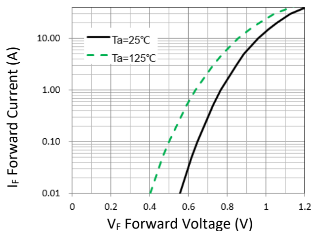
Figure 1. Forward Characteristic(typ.)
