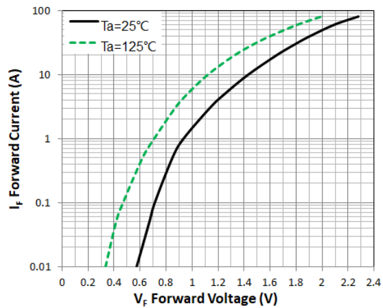
Figure 1. Forward Characteristic(typ.)
