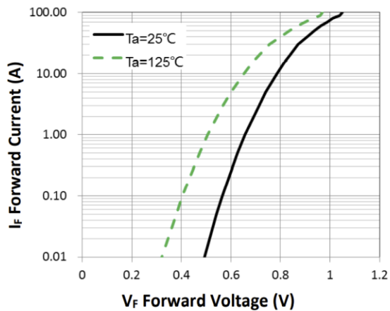
Figure 1. Forward Characteristic(typ.)
