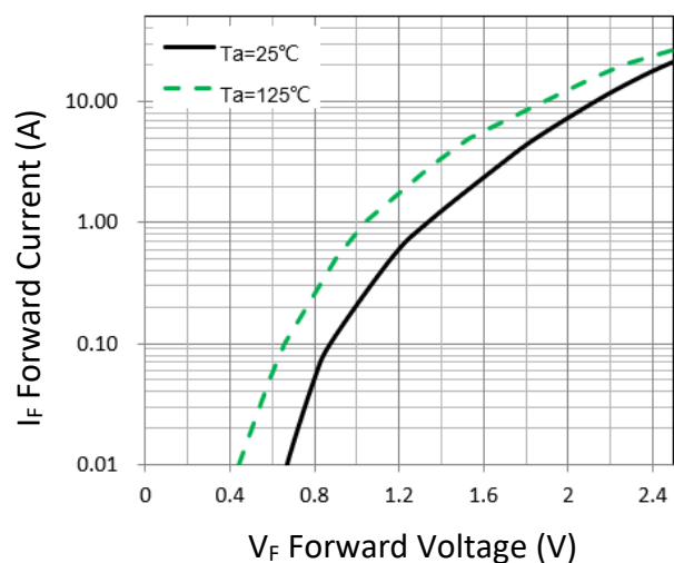
Figure 1. Forward Characteristic(typ.)
