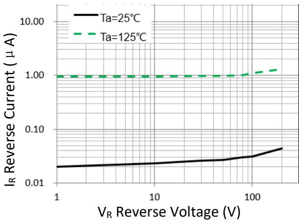
Figure 2. Reverse Characteristic (typ.)
