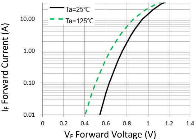
Figure 1. Forward Characteristic(typ.)
