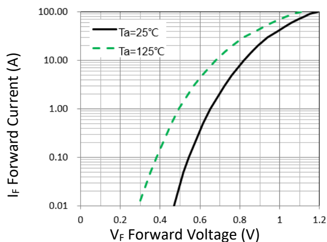
Figure 1. Forward Characteristic(typ.)
