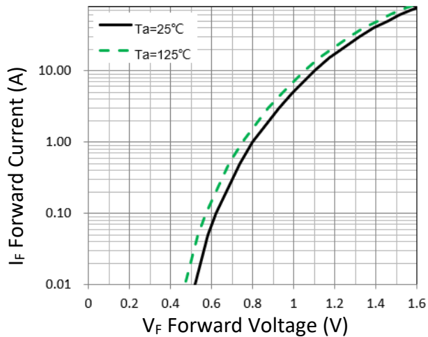
Figure 1. Forward Characteristic(typ.)
