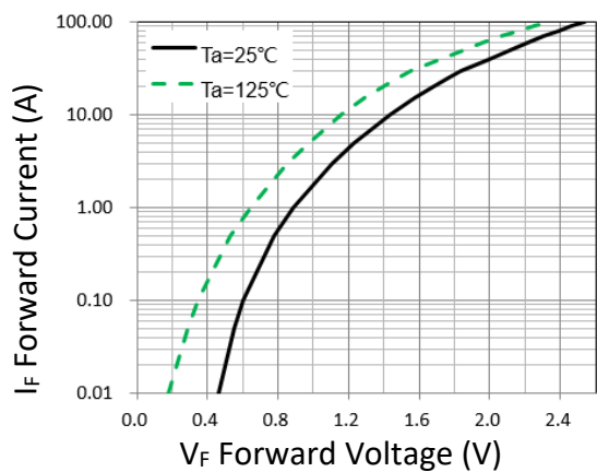
Figure 1. Forward Characteristic(typ.)
