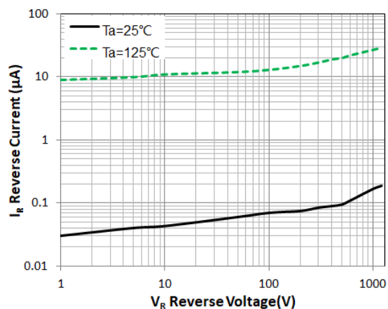
Figure 2. Reverse Characteristic(typ.)
