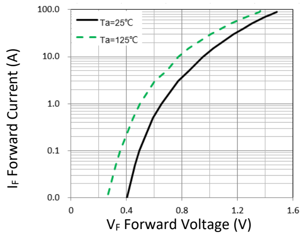
Figure 1. Forward Characteristic(typ.)
