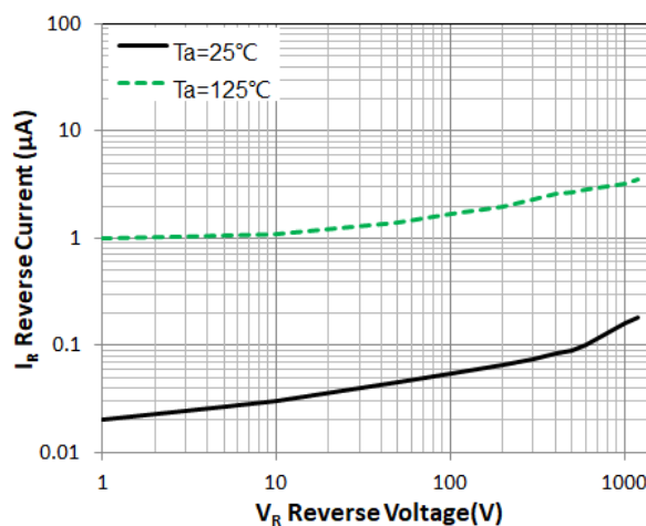
Figure 2. Reverse Characteristic(typ.)
