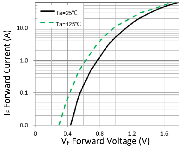
Figure 1. Forward Characteristic(typ.)
