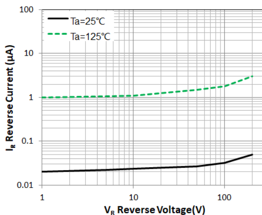
Figure 2. Reverse Characteristic(typ.)
