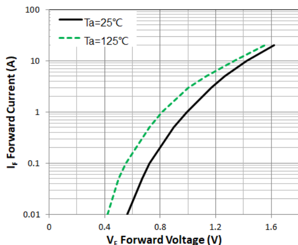
Figure 1. Forward Characteristic(typ.)
