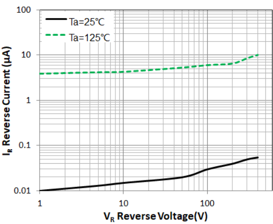
Figure 2. Reverse Characteristic(typ.)
