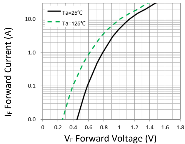
Figure 1. Forward Characteristic(typ.)
