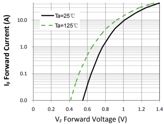
Figure 1. Forward Characteristic(typ.)
