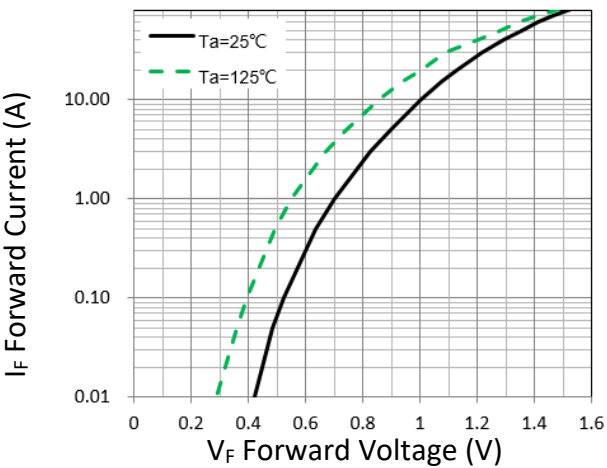
Figure 1. Forward Characteristic(typ.)
