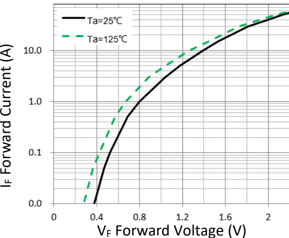
Figure 1. Forward Characteristic(typ.)
