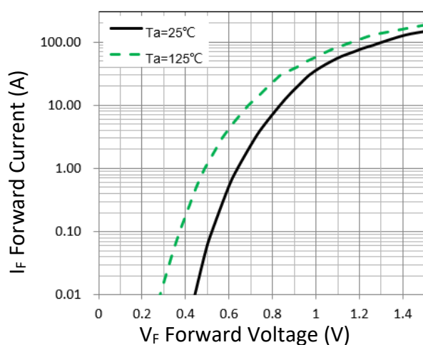
Figure 1. Forward Characteristic(typ.)
