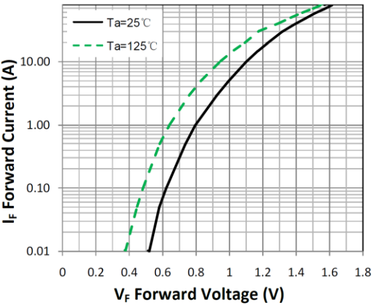
Figure 1. Forward Characteristic(typ.)
