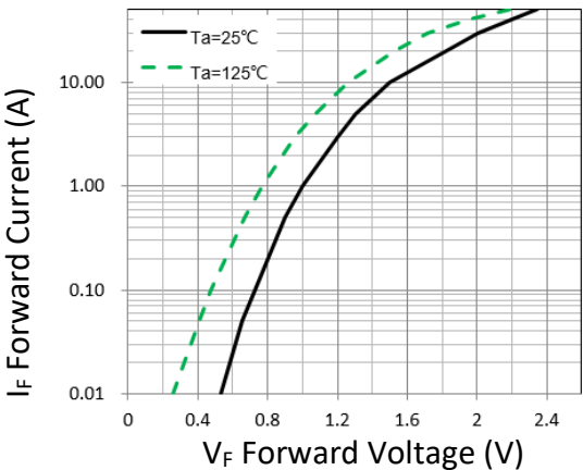
Figure 1. Forward Characteristic(typ.)
