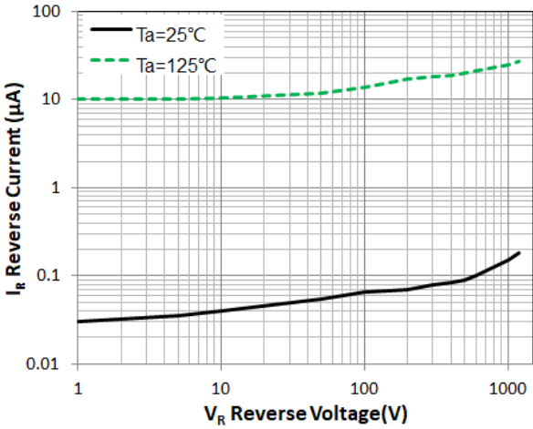
Figure 2. Reverse Characteristic(typ.)
