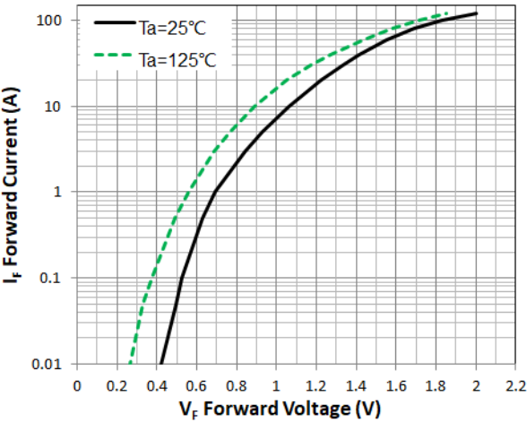
Figure 1. Forward Characteristic(typ.)
