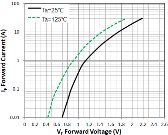
Figure 1. Forward Characteristic(typ.)
