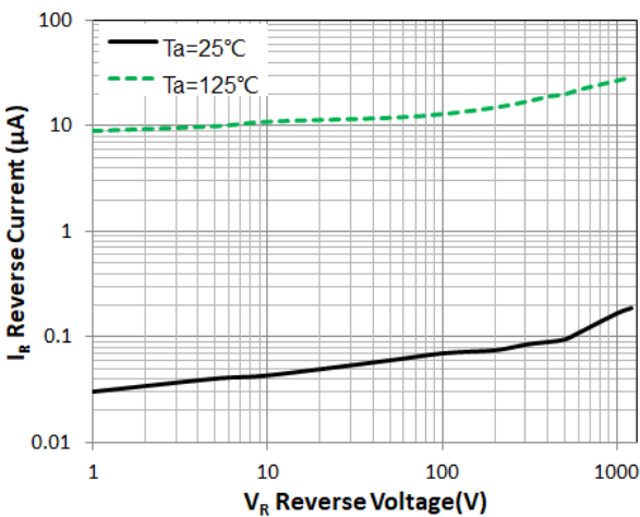
Figure 2. Reverse Characteristic(typ.)
