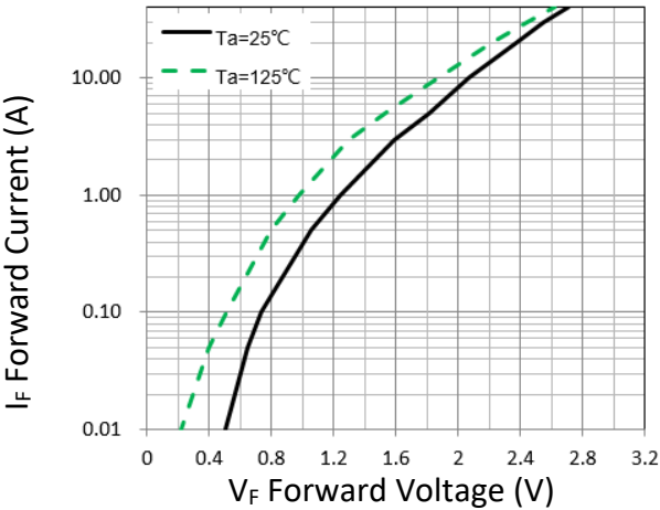
Figure 1. Forward Characteristic(typ.)
