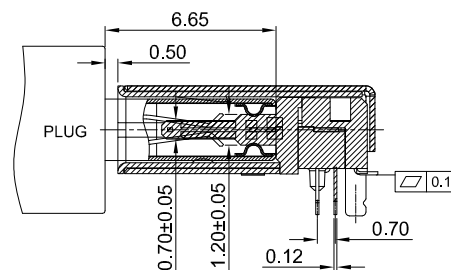
SECTION A-A AFTER MATING
