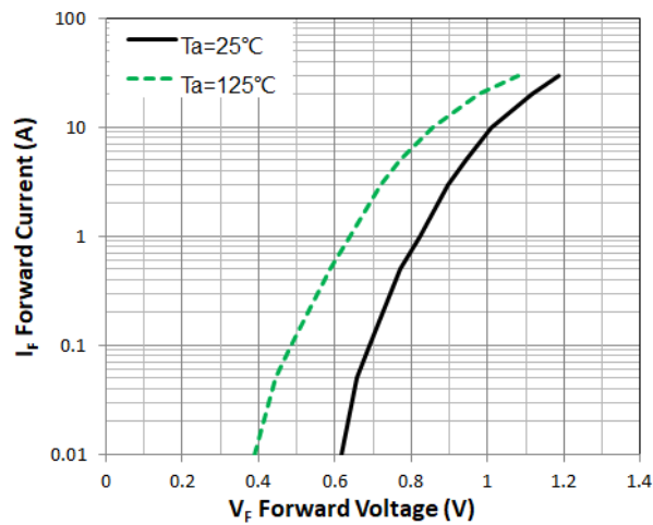
Figure 1. Forward Characteristic(typ.)
