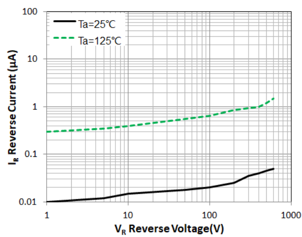
Figure 2. Reverse Characteristic(typ.)
