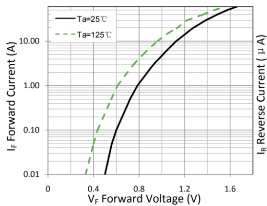
Figure 1. Forward Characteristic(typ.)
