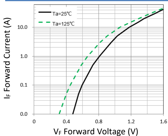
Figure 1. Forward Characteristic(typ.)
