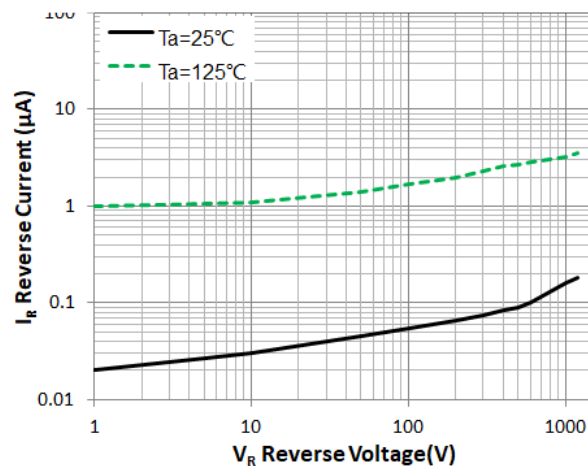
Figure 2. Reverse Characteristic(typ.)
