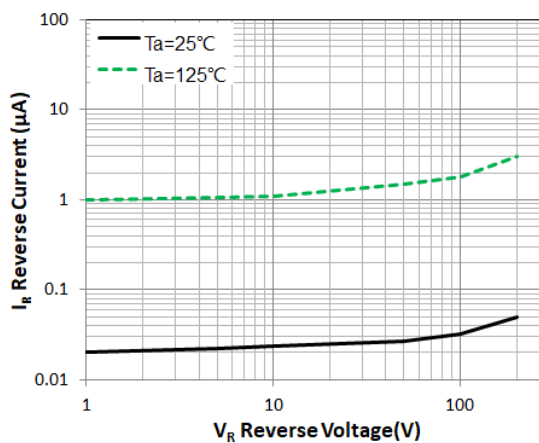
Figure 2. Reverse Characteristic(typ.)
