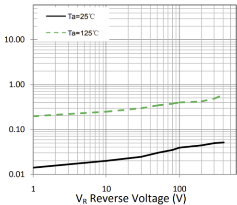
Figure 2. Reverse Characteristic (typ.)
