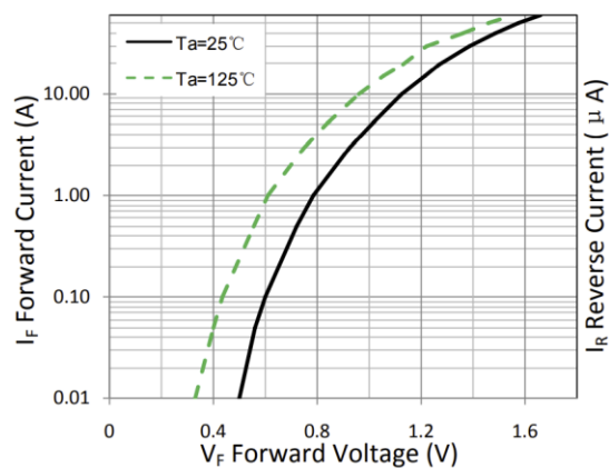
Figure 1. Forward Characteristic(typ.)
