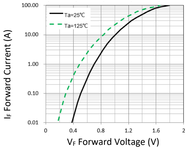
Figure 1. Forward Characteristic(typ.)
