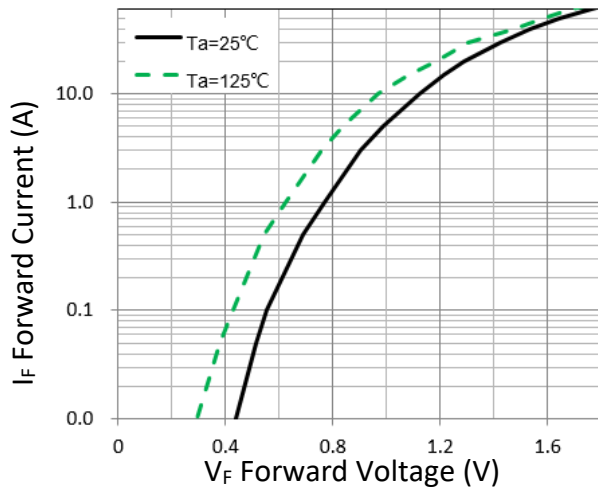
Figure 1. Forward Characteristic(typ.)
