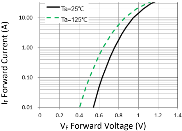
Figure 1. Forward Characteristic(typ.)
