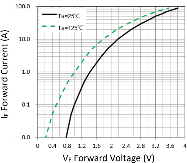
Figure 1. Forward Characteristic(typ.)
