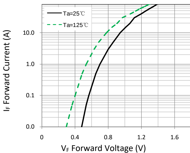
Figure 1. Forward Characteristic(typ.)
