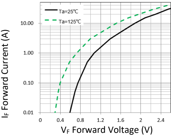
Figure 1. Forward Characteristic(typ.)
