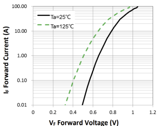
Figure 1. Forward Characteristic(typ.)
