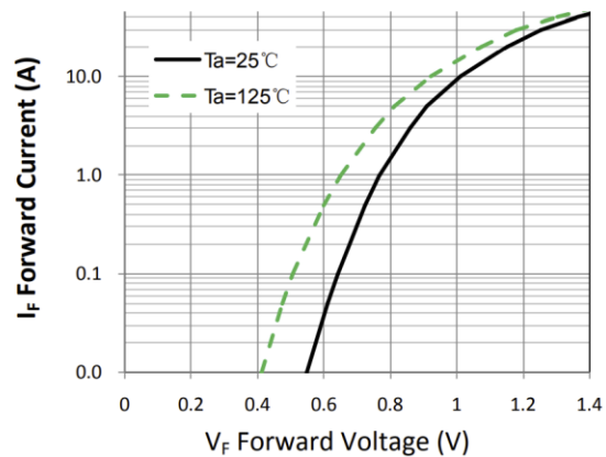
Figure 1. Forward Characteristic(typ.)
