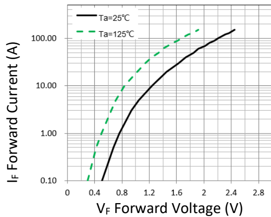
Figure 1. Forward Characteristic(typ.)
