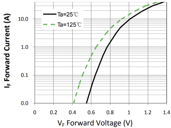
Figure 1. Forward Characteristic(typ.)
