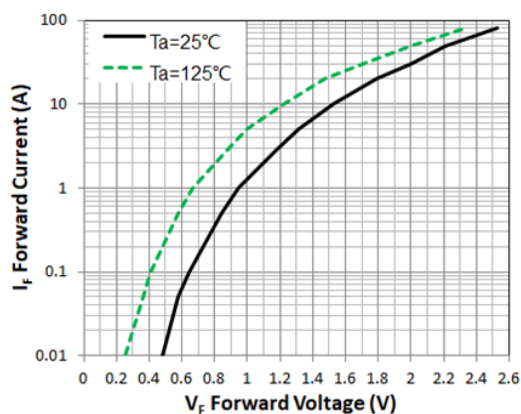
Figure 1. Forward Characteristic(typ.)
