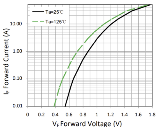
Figure 1. Forward Characteristic(typ.)
