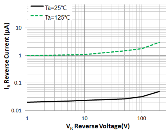
Figure 2. Reverse Characteristic(typ.)
