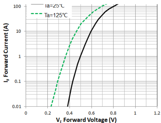
Figure 1. Forward Characteristic(typ.)
