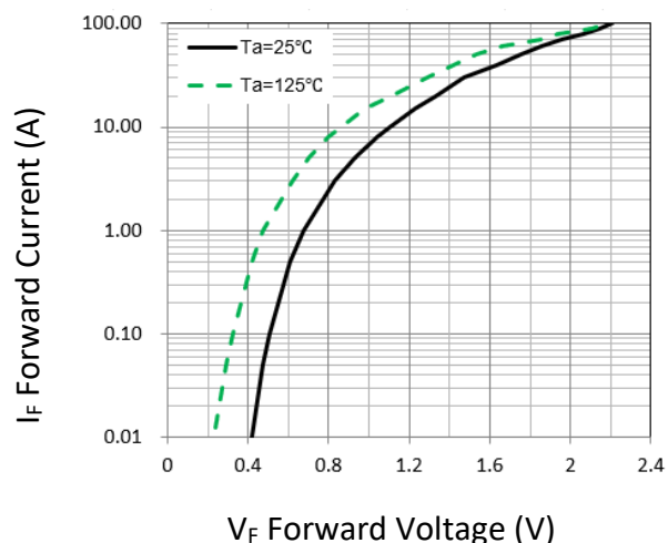
Figure 1. Forward Characteristic(typ.)
